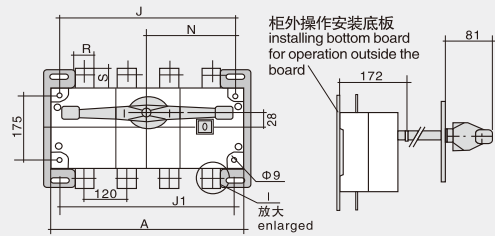
XLGL-1000~1600A/J柜外操作 operation outside XLGL-1000~1600A/J board
