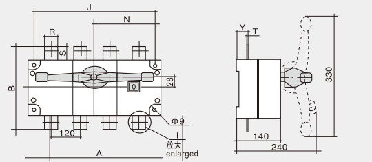
XLGL-1000~1600A直接操作 Direct operation of HGL-1000~1600A
