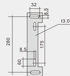
柜外操作安装底板 Installation bottom board for operation outside the board
