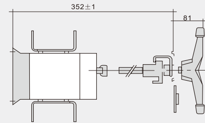
XLGL-2000~2500A正面柜外操作 operation outside HGL-2000~2500A
