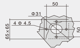
XLGL-2000~2500A正面柜外操作 operation outside HGL-2000~2500A
